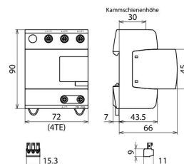
Dimension drawing DV M2 TNC 255 FM
